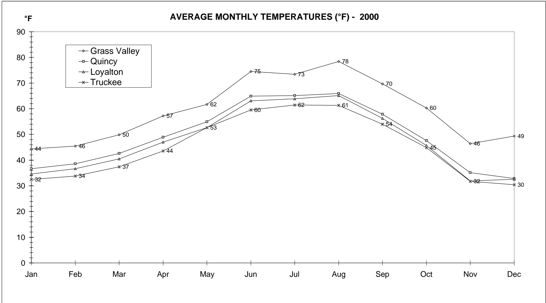
Average Monthly Temperatures (°F): 1996 - 2000
